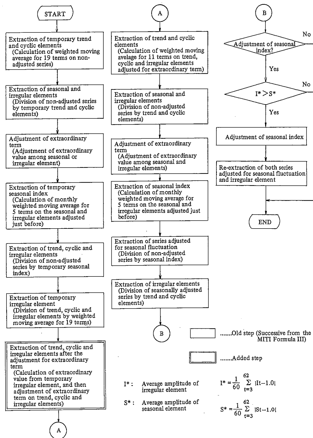
Block Chart of the MITI Formula III R (excluding the part of analysis calculation)
